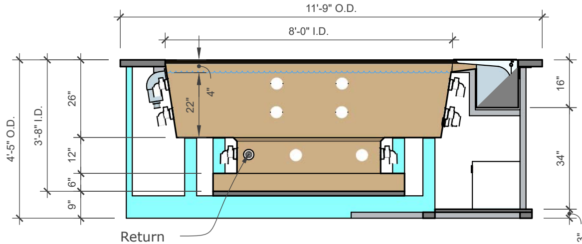
SECTION 3 SECTION SCALE 3/8" = 1'
