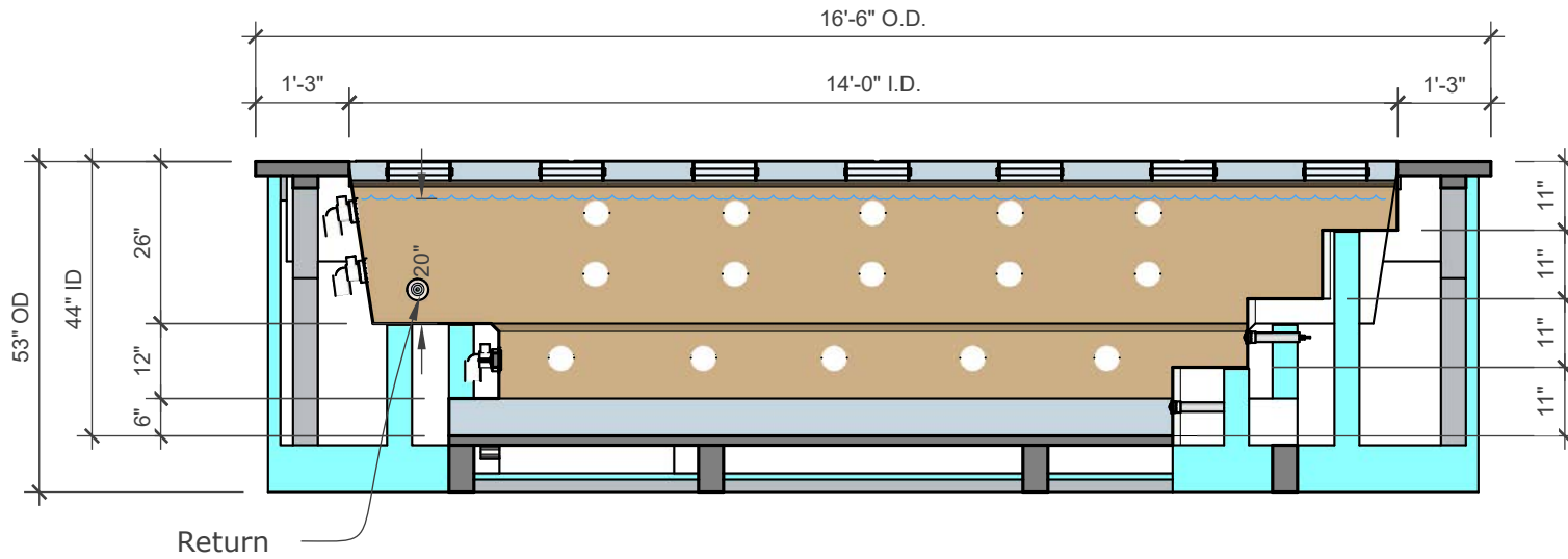
SECTION 4 SECTION SCALE 3/8" = 1'
