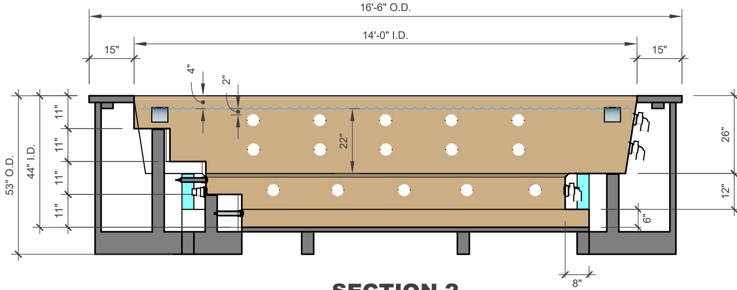
SECTION 2 SECTION SCALE 3/8" = 1'
