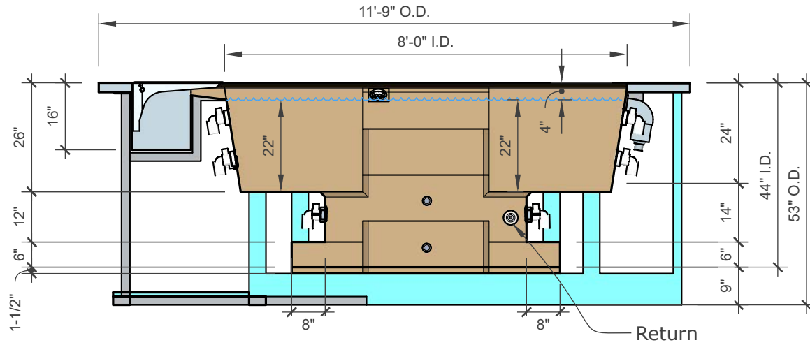
SECTION 1 SECTION SCALE 3/8" = 1'
